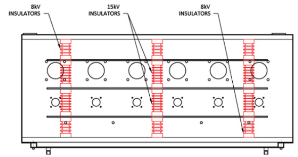
TOP SECTION-THROUGH
